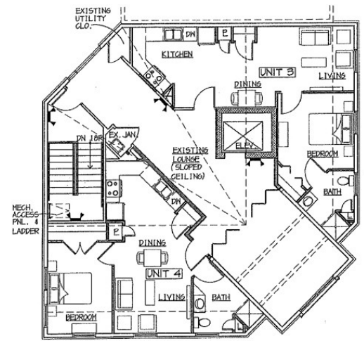
PROPOSED SECOND FLOOR
